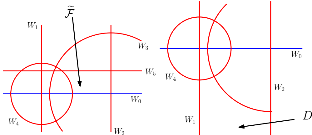
FIGURE 4. The regions \tilde{\mathcal{F}} and D in the proof of Theorem 3
