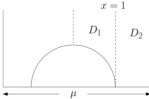
FIGURE 3. The regions D_1 and D_2 in the proof of Theorem 4
